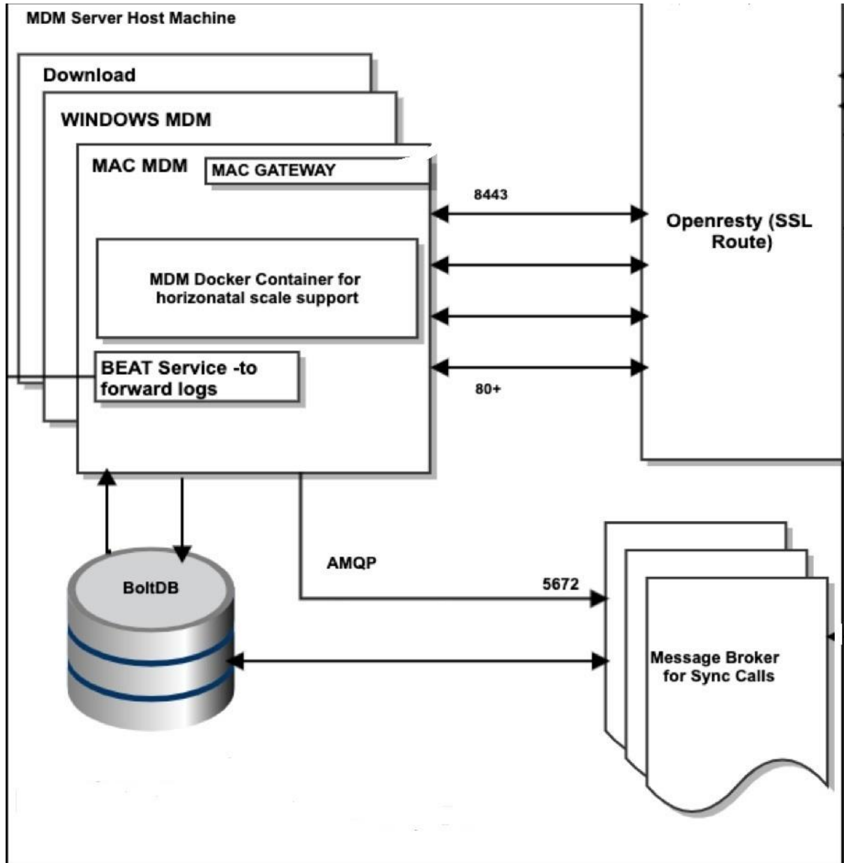
Figure 18: MDM Server Docker Host
