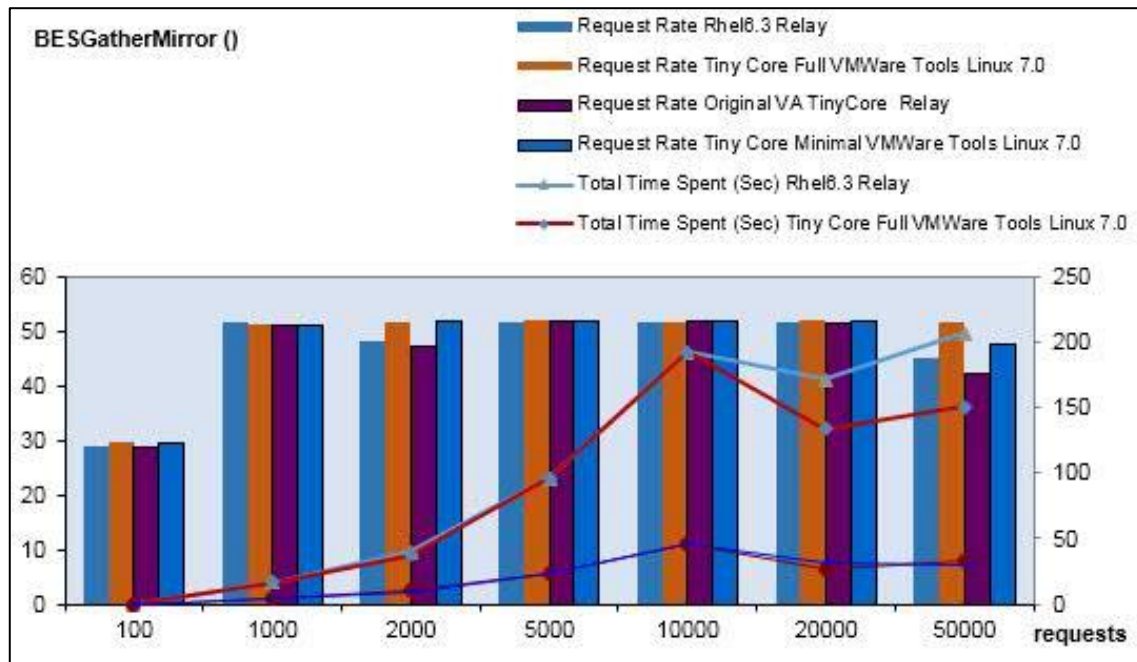
Figure 16: BigFix Relay Virtualization Performance
